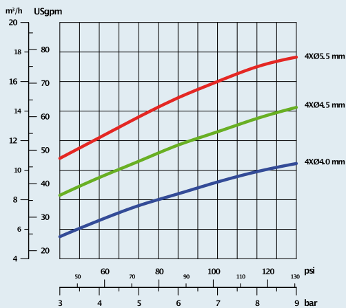
Pressure/Flow
